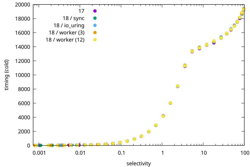
uniform / indexscan / eic=16
