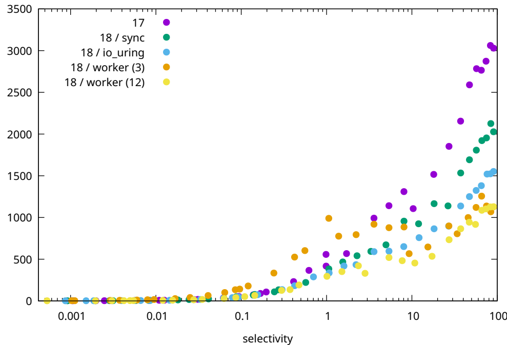
uniform / bitmapscan / eic=16
