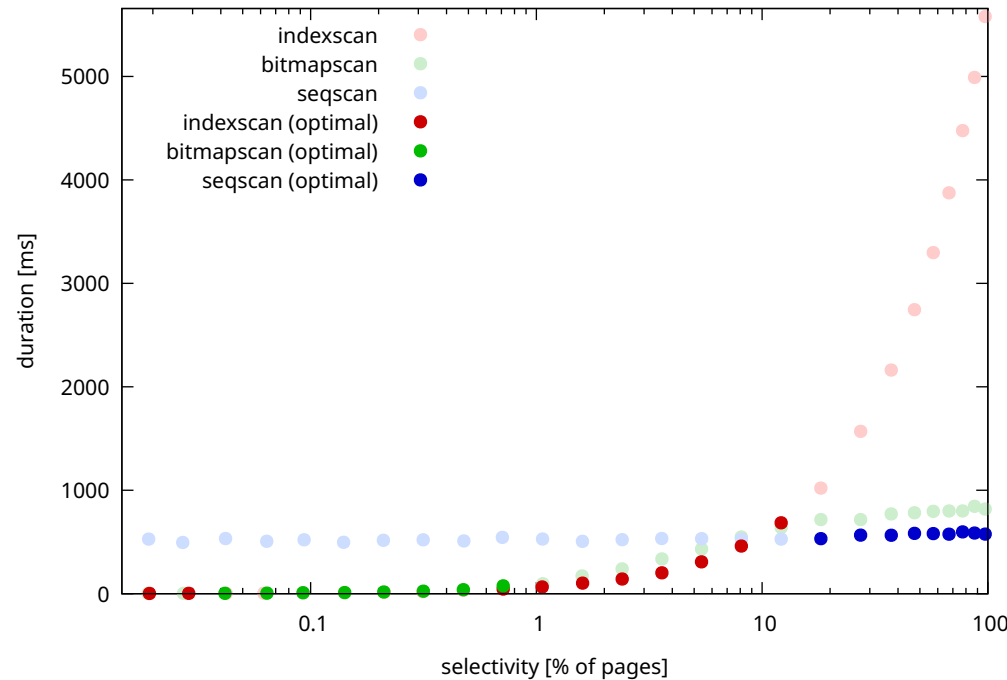
timing (warm) / uniform / random_page_cost=1.25
