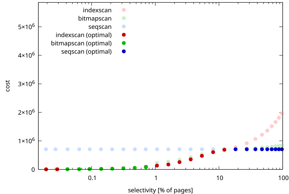
cost estimate / uniform / random_page_cost=1.25
