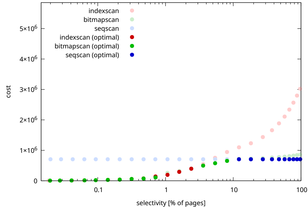
cost estimate / uniform / random_page_cost=2
