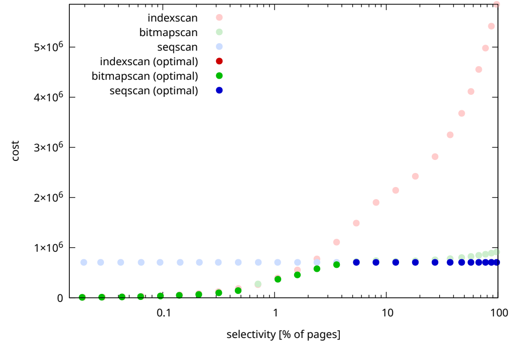
cost estimate / uniform / random_page_cost=4
