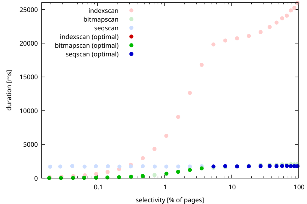
timing (cold) / uniform / random_page_cost=4
