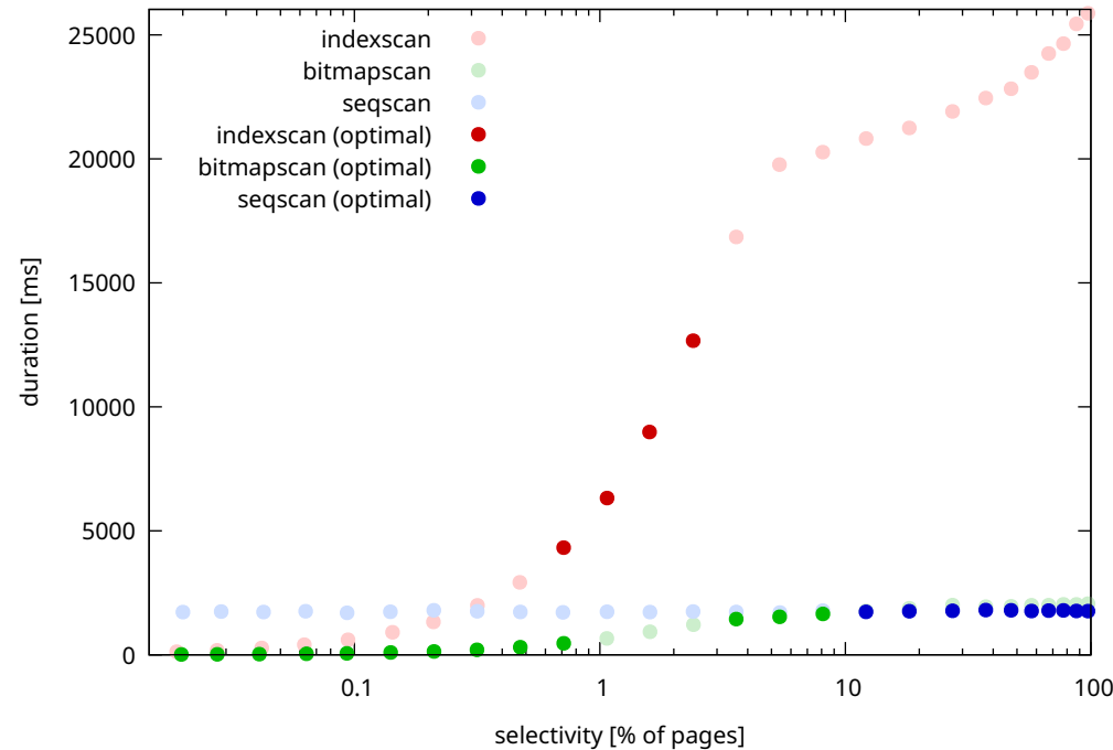
timing (cold) / uniform / random_page_cost=2
