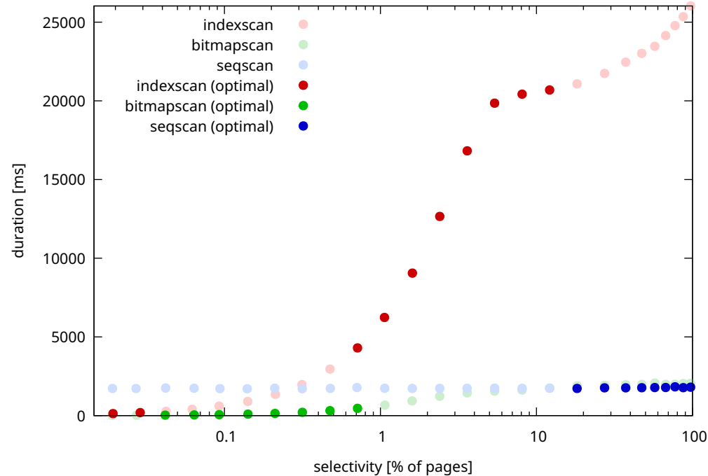
timing (cold) / uniform / random_page_cost=1.25
